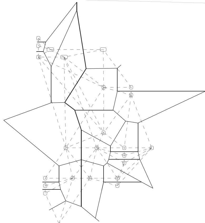
VORONOI DIAGRAM
